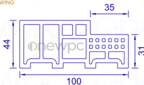
CROSS-SECTIONAL AREA
