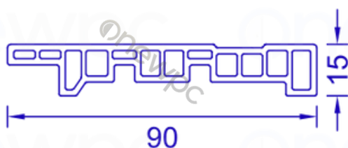
CROSS-SECTIONAL AREA
