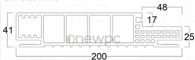
TECHNICAL DRAWING
