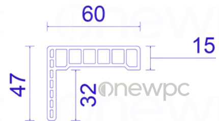
TECHNICAL DRAWING
