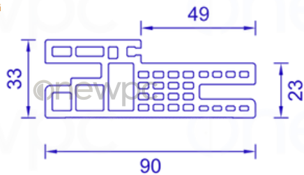
TECHNICAL DRAWING
