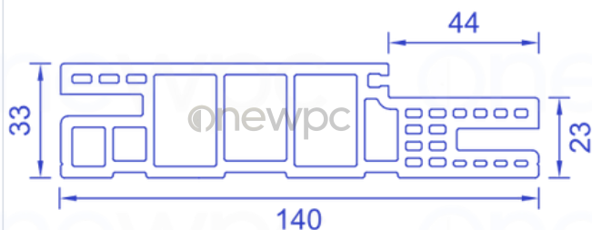
TECHNICAL DRAWING
