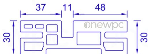
CROSS-SECTIONAL AREA
