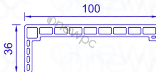
CROSS-SECTIONAL AREA
