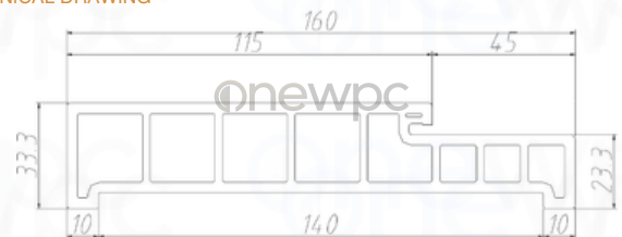
CROSS-SECTIONAL AREA
