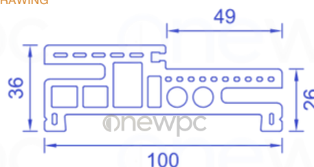
CROSS-SECTIONAL AREA
