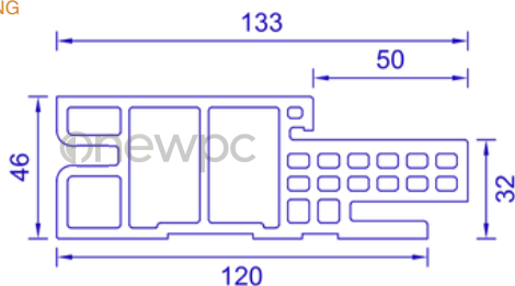
TECHNICAL DRAWING
