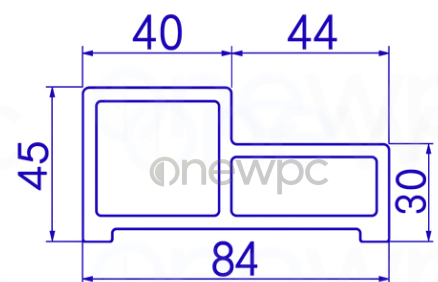
TECHNICAL DRAWING
