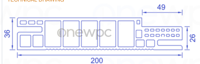
TECHNICAL DRAWING
