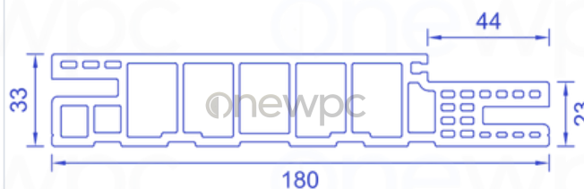
TECHNICAL DRAWING
