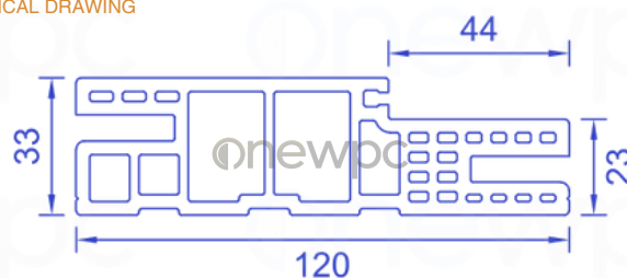
CROSS-SECTIONAL AREA
