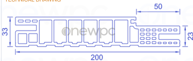
TECHNICAL DRAWING
