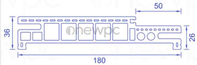
TECHNICAL DRAWING
