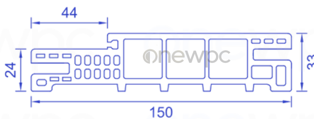
TECHNICAL DRAWING
