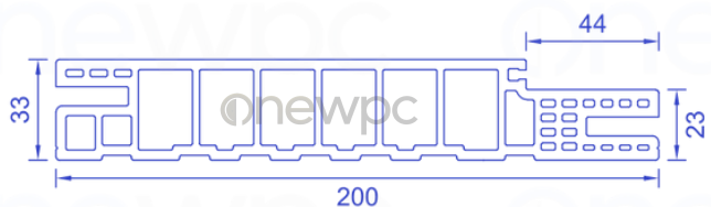
TECHNICAL DRAWING
