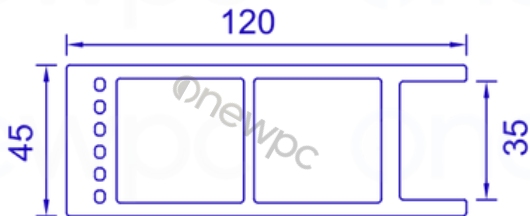
CROSS-SECTIONAL AREA
