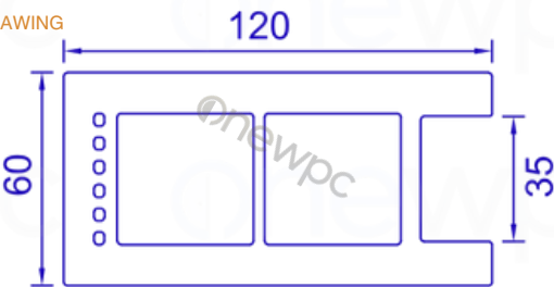
CROSS-SECTIONAL AREA
