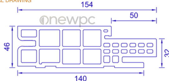
CROSS-SECTIONAL AREA
